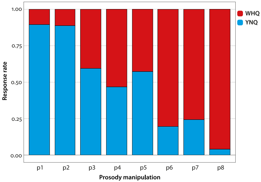
Figure 10. Response rate for YNQ-based stimuli
