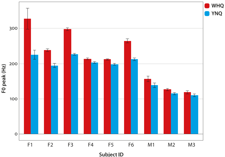
Figure 5. The F0 peaks of the wh -word
