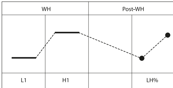
Figure 6. Canonical intonational contours of (a) YNQ and (b) WHQ
