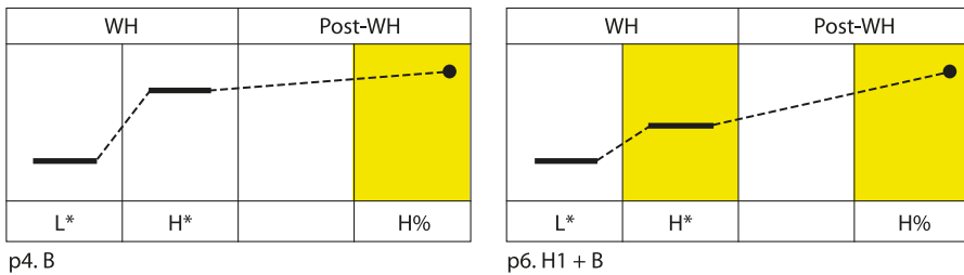
Figure 13. Schematic representation of some WHQ-based stimuli
