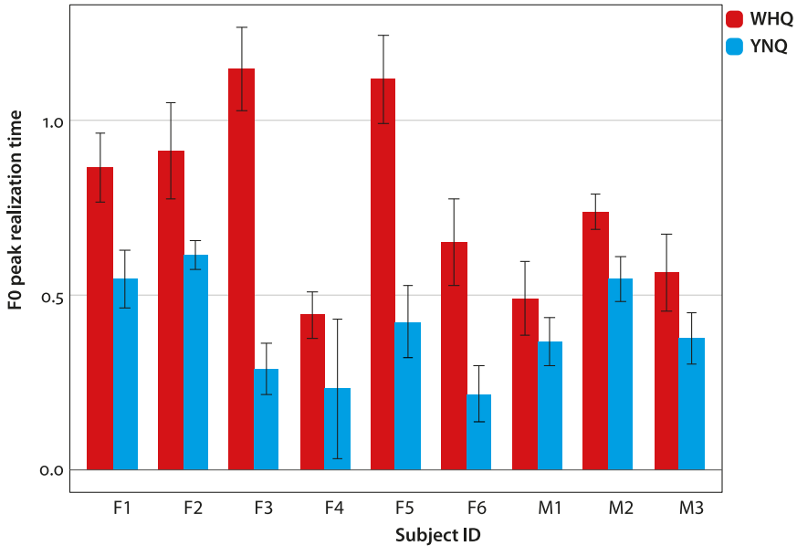
Figure 12. Timing of the F0 peak realization from the onset of the second vowel of the wh -word. o indicates the starting point of the vowel, and l indicates the ending point
