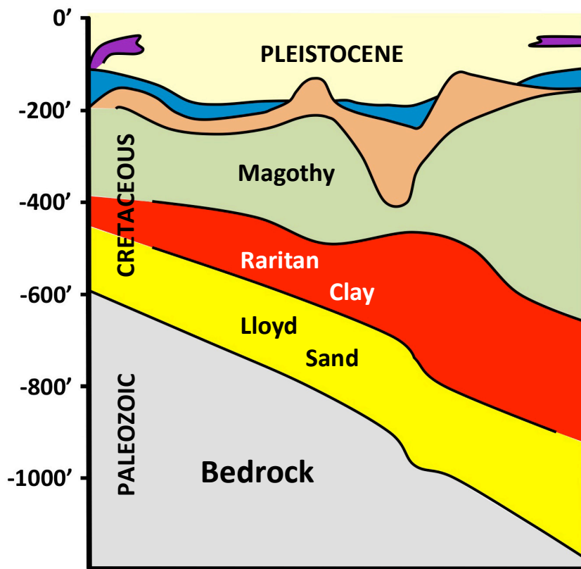
Figure 2 – Strata Along the South Shore of Brooklyn and Queens. Paleozoic metamorphic bedrock is covered with layers of Cretaceous coastal plains sand and clay. The regional bedrock/Cretaceous soil surface was carved by erosion, leaving behind valleys and scattered depressions that were filled and covered over with Pleistocene deposits. The cross-section is compiled from multiple U.S.G.S. map resources to reflect general stratigraphy along the southern edge of NYC (yellow line).
