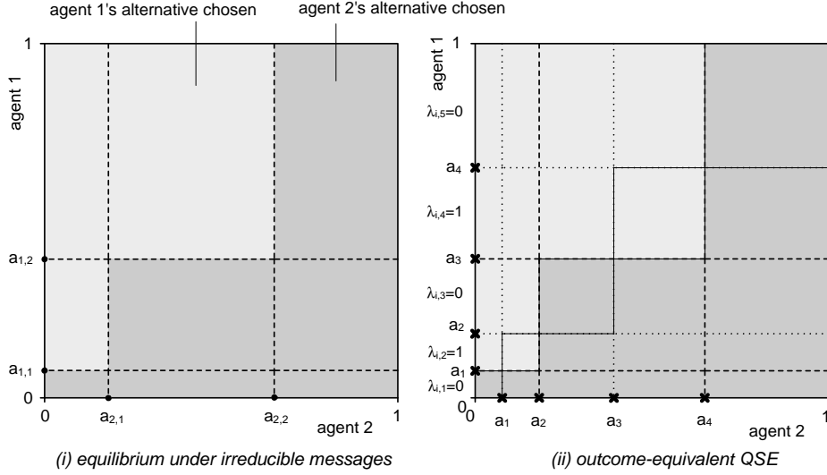
Figure 3: Outcome-equivalence between QSE and irreducible messages
