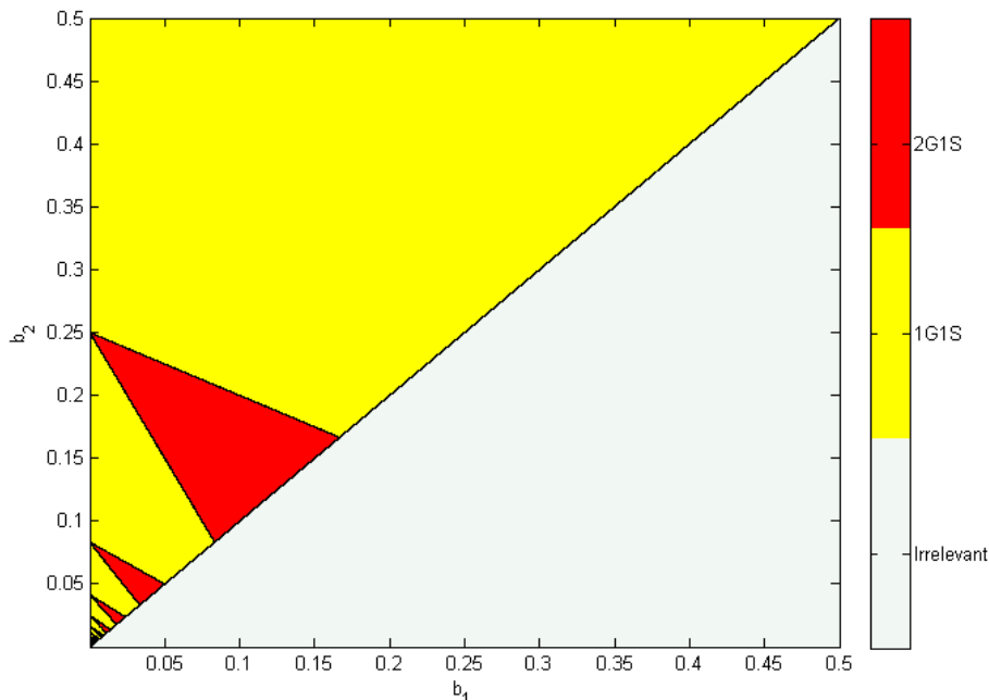
Figure 7: The Most Informative Equilibrium and the Biases
