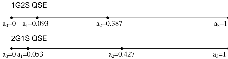
Figure 5: 1G2S QSE and 2G1S QSE
